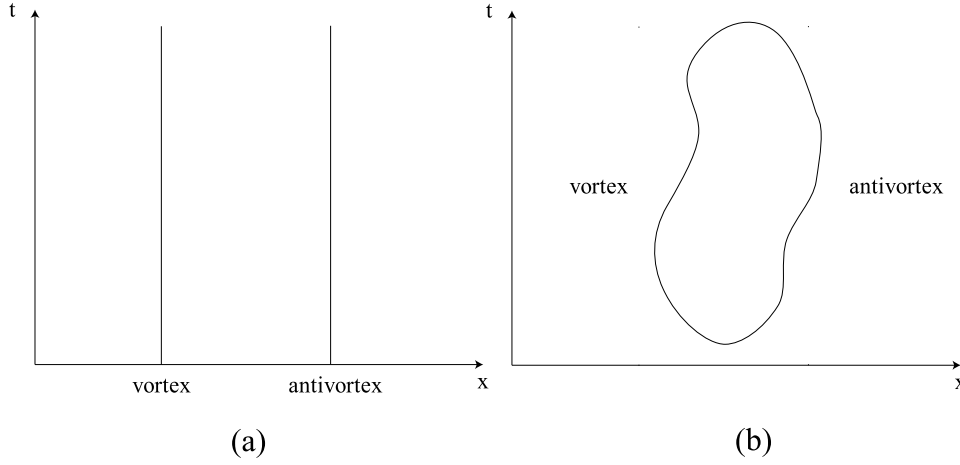
FIGURE 1. Time evolution of a vortex-antivortex pair
